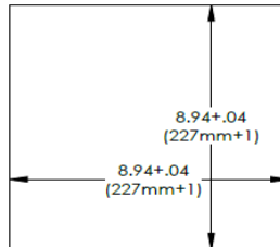
CUT-OUT DIAGRAM
