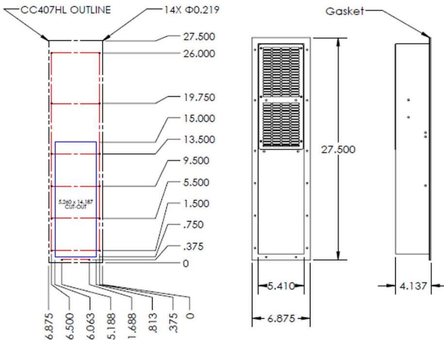
CABINET HOLE PATTERN (EXTERNAL VIEW)
